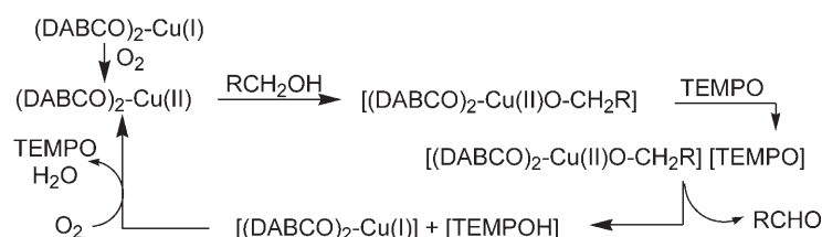
Figure 3. Proposed catalytic cycle for the oxidation of alcohols using DABCO-CuCl-TEMPO complex.
