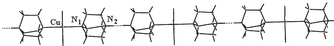
Figure 2. Linear polymeric structure of the DABCO-Cu complex due to strong intermolecular hydrogen bonding.
