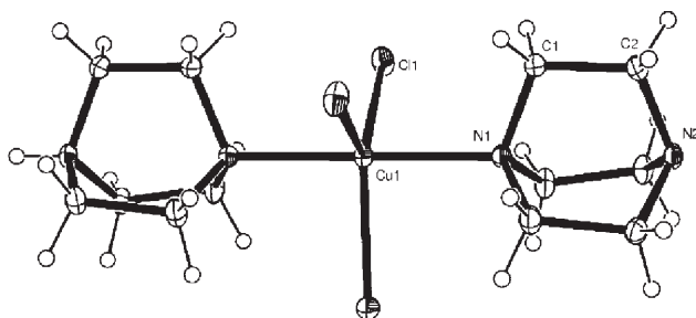
Figure 1. Solid-state structure determination of the DABCO-Cu complex (30% probability; CCDC No.: 633455).
